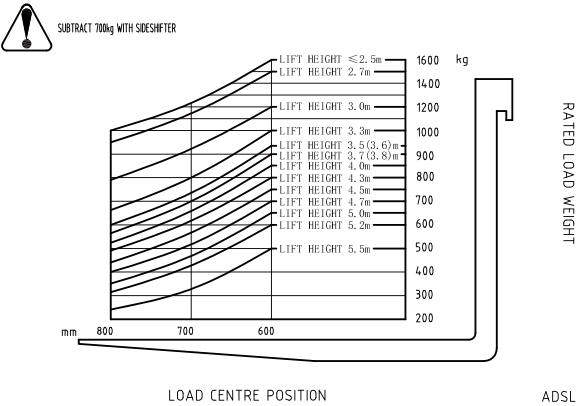
RATED CAPACITIES AND LOAD CENTRES GRAPH
