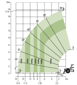
Range of Motion ZTH4014
