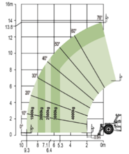
Range of Motion ZTH4014
