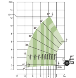
Range of Motion ZTH4018
